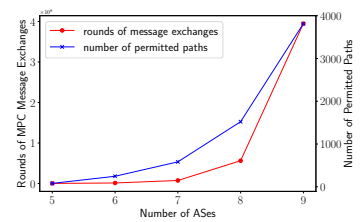
Fig. 7: Rounds of communications performed by P-GREEDYMIS protocol.
