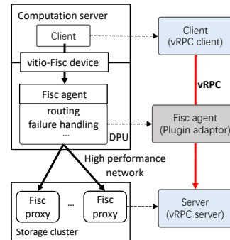
Figure 6: The abstracted vRPC.
